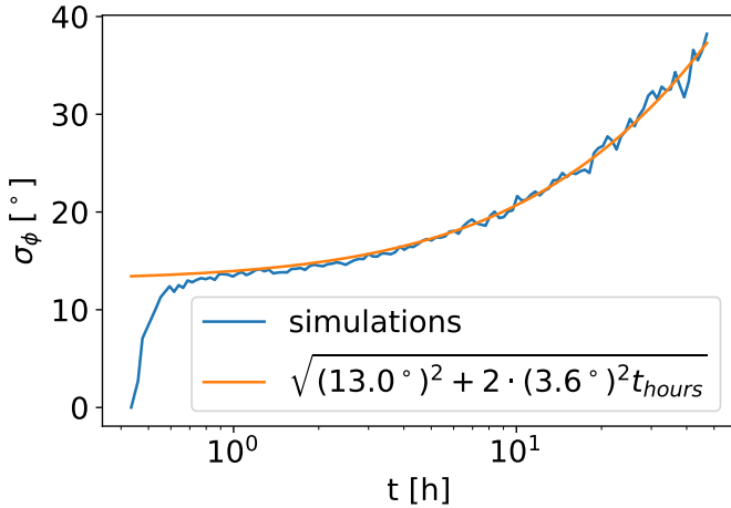
Fig. 4. Heliongitudinal standard deviation of the 100-MeV protons as a function of time. The amber curve shows the functional form where the standard deviation is initially 13^\circ , and then increases consistent with longitudinal diffusion with diffusion coefficient \kappa_\phi = (3.6^\circ)^2/\text{h} .
