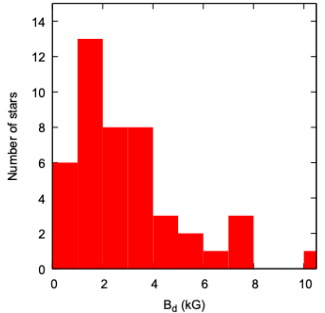
Fig. 5. Distribution of the magnetic dipole field strength B_d for the Ap stars of the volume-limited sample of Sikora et al. (2019b).
