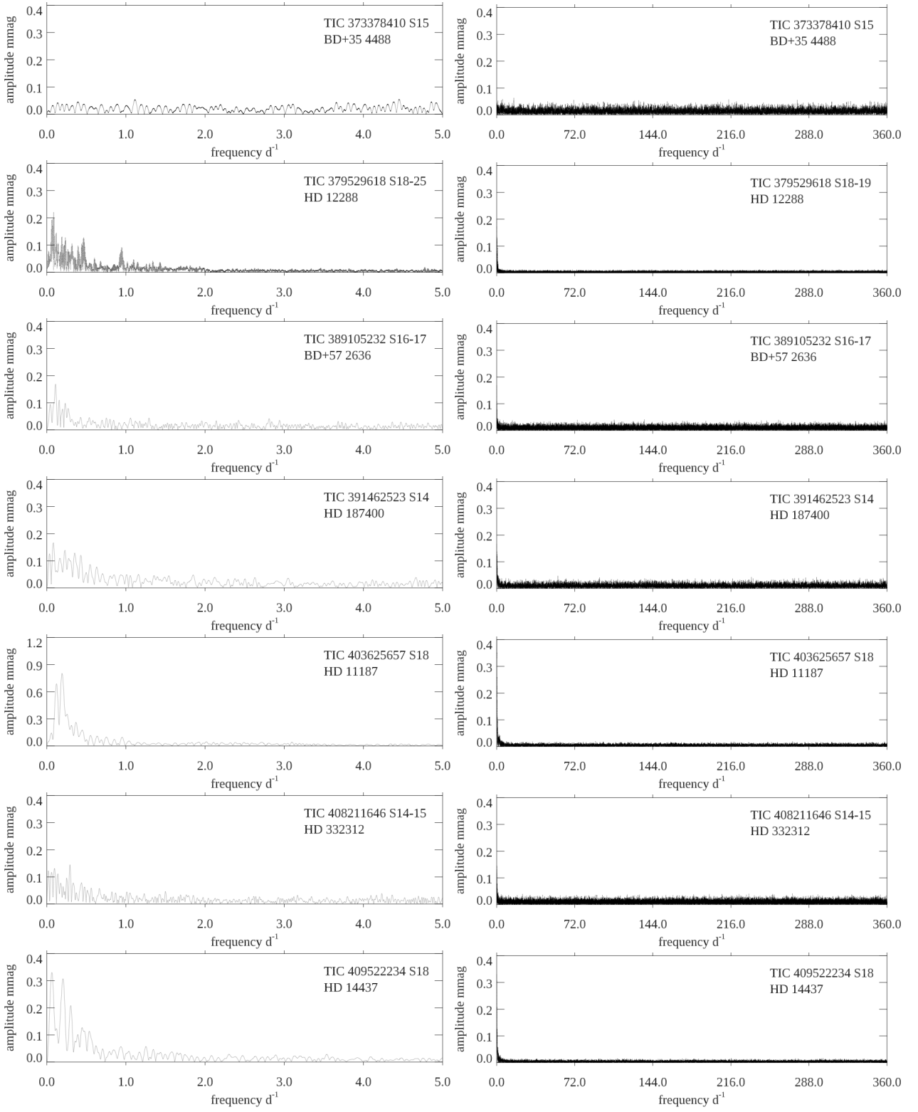
Fig. B.8. Amplitude spectra for the long-period Ap stars, continued. TIC 379529618 shows some low-frequency variability that is not rotational. The peak at 0.96 \text{d}^{-1} is coherent across two sectors, but does not appear in the third sector. It is of unknown origin.
