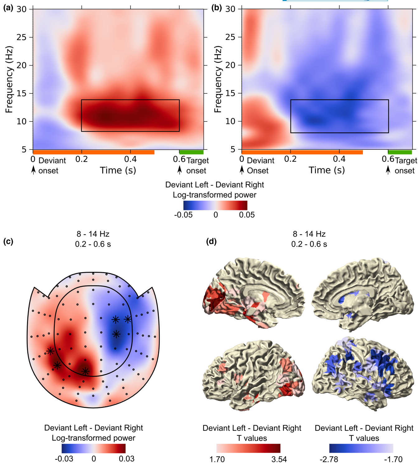
FIGURE 3 Log10-transformed alpha power modulation to lateralized deviants based on group-averaged data for Deviant Left minus Deviant Right. (a and b) Time–frequency representations highlighting (a) high alpha power ipsilateral to the deviant location at left-hemispheric posterior gradiometers (average across three channels showing a prominent effect, marked in C with a star), and (b) low alpha power contralateral to the deviant location at right-hemispheric centro-temporal gradiometer (average across three channels showing a prominent effect, marked in C with a star). The black box marks the time–frequency range (time: 0.2–0.6 s, frequency: 8–14 Hz) used for the statistical cluster analysis. (c) Topoplot of the alpha power distribution in the 0.2–0.6 s time window following deviant onset. Stars indicate channels on which there was a prominent statistical effect. (d) Source estimation of the alpha power effects. Note that the data were not baseline corrected.
