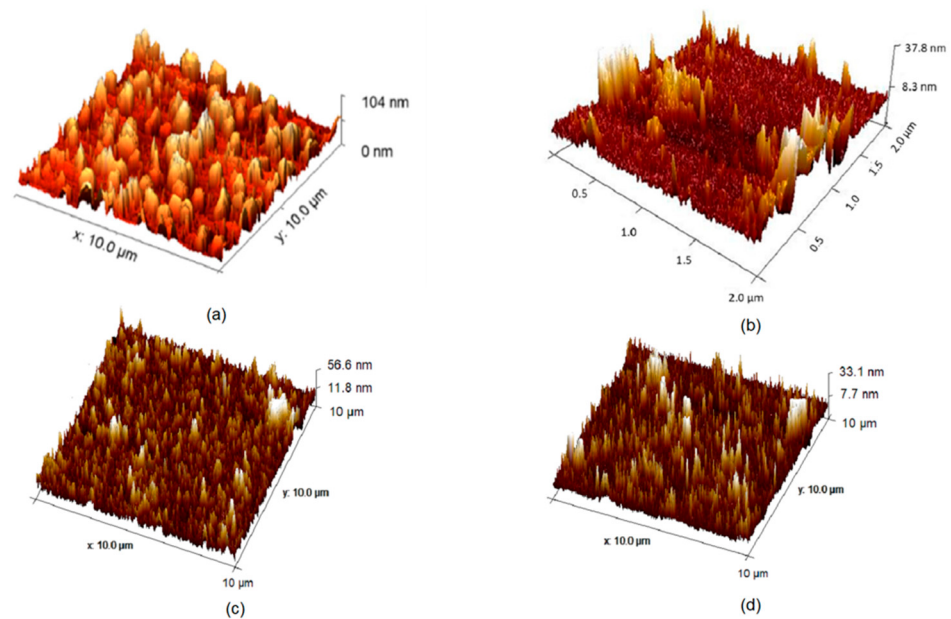
Figure 2. AFM of QCM-D crystals coated with: (a) Nafion, (b) (Naf/Lys) 6 , (c) (Naf/CDot) 6 , and (d) (Naf/Lys/CDot/Lys) 3 . Subscript number refers to the number of bi- or trilayers. (a,b) adapted from [23].
