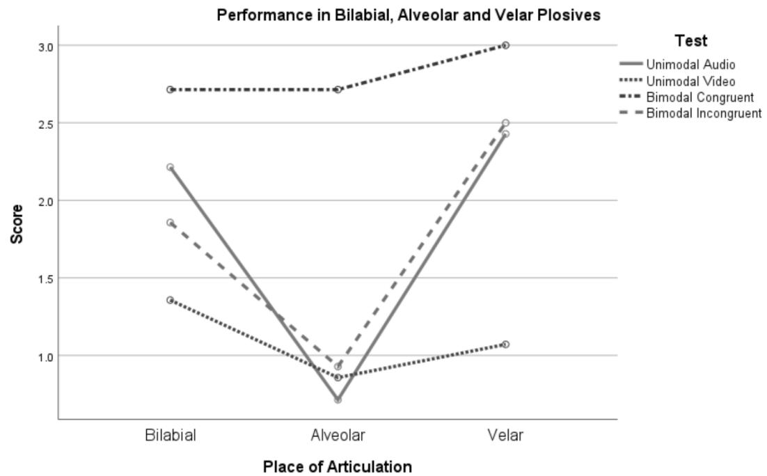
Figure 3. Mean score of participants in target bilabial, alveolar and velar plosives in each condition
