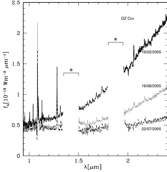
Figure 2. NTT time-series spectra of DZ Cru in the JHK bands (0.95–2.52 \mu\text{m} ), spanning from 2005 February 16 to 2005 July 22 UT ( \sim 1.5 –2 yr from maximum brightness). Gaps in the data in the \sim 1.34 – 1.50 and \sim 1.80 – 1.95 \mu\text{m} regions are owing to strong absorption from terrestrial \text{H}_2\text{O} . Identifications of the spectral lines are given in Fig. 3. Date format is DD/MM/YY.
