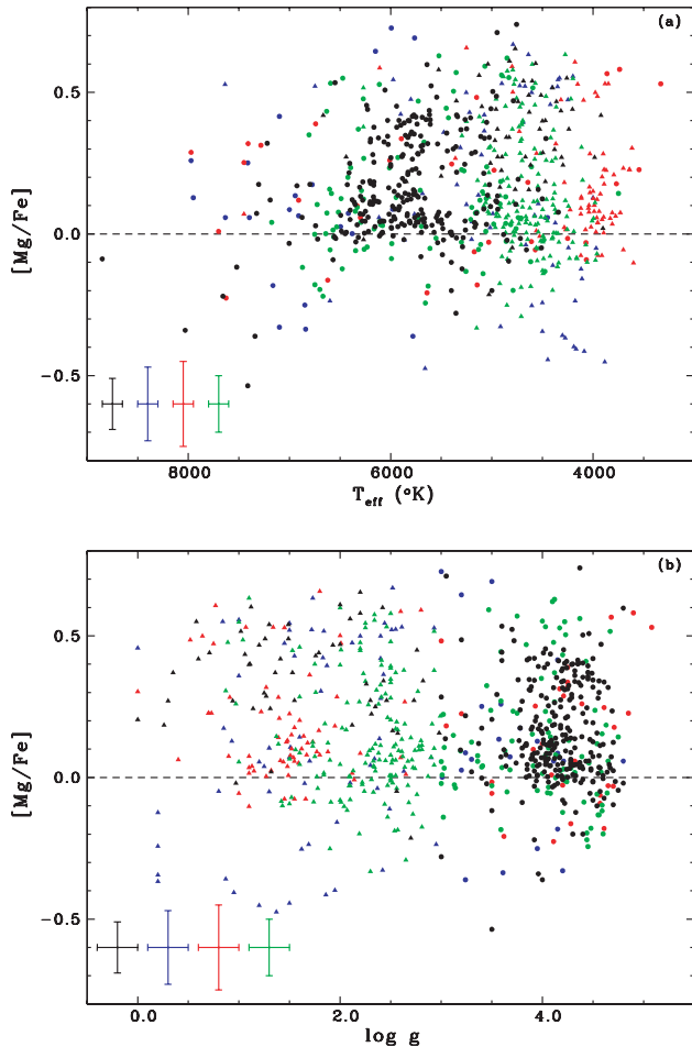
Figure 11. Distribution of [Mg/Fe] in our catalogue over the scales of effective temperature (truncated at 9000 K) in the top panel (a), and surface gravity in the bottom panel (b). The notations are those adopted in Fig. 10.
