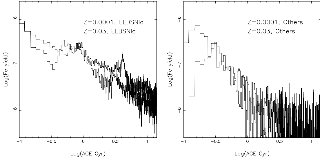
Figure 4. Time evolution of iron yields from two different groups of SNIa, from binary-star model yields. The models shown are for ELD and other SNIa as listed in Table 3.
