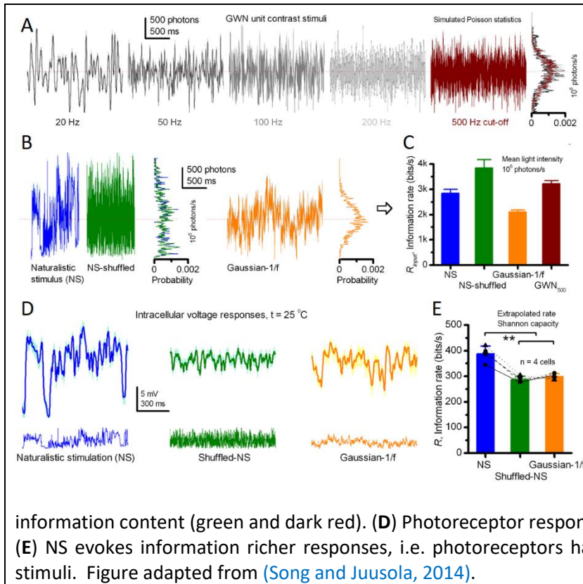
Fig. 5. The Naturalistic Stimuli generate larger and information-richer photoreceptor responses than the artificial stimuli, highlighting the importance of temporal correlations in naturalistic stimuli. (A) GWN stimuli with different frequency cut-offs. (B) Three types of manipulated NS stimuli. Blue: a naturalistic stimulus time series (NS) selected from van Hateren natural stimulus collection. Green: a shuffled-NS, in which all the NS intensity values are rearranged in a random order, effectively whitening the Orange: an artificial GWN-1/f stimulus, which is a random phase-shifted NS. (C) Whitened stimuli have higher
