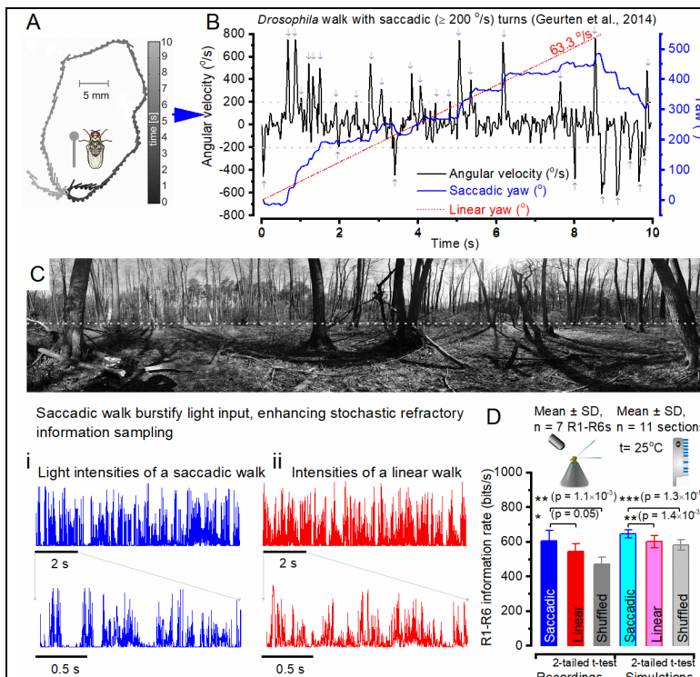
Fig. 6. A Drosophila's saccadic walk generates a bursty high-contrast time series from natural scenes, enabling its photoreceptor to extract more information from the environment than other walking patterns, including linear scanning. (A-B) Angular velocity and yaw of a prototypical walking trajectory (Geurten et al., 2014). (C) A natural scene used for generating light intensity time series: (i) by translating the saccadic yaw (A-B) dynamics on it (blue trace), and (ii) by a linear walk with the median velocity of the saccadic walk. (D) Saccadic walk enables an R1-R6 photoreceptor to capture more information from the environment. The darker bar colours (left) indicate intracellular in vivo photoreceptor
