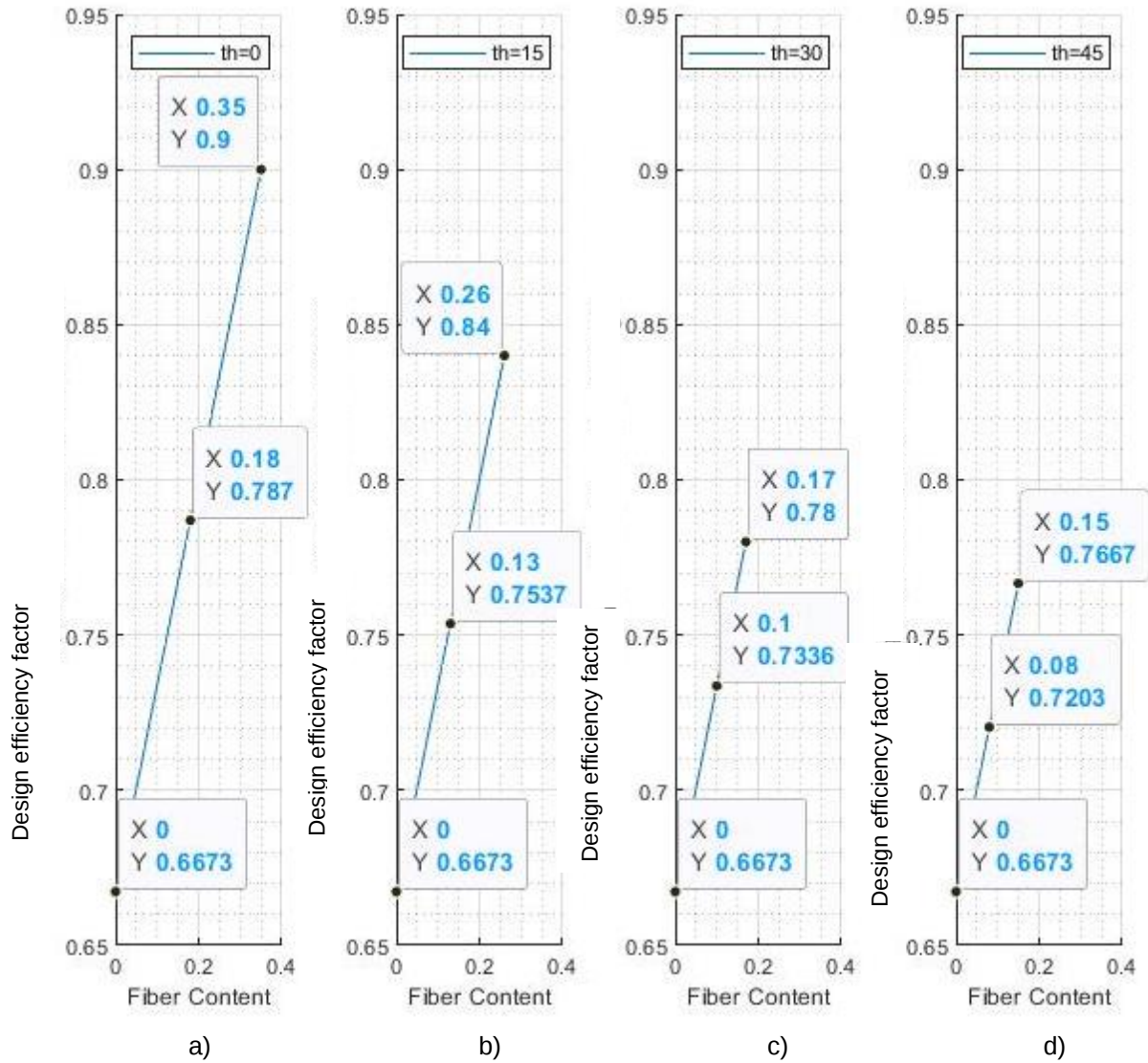
Figure 9: Design efficiency factor vs fiber volume content for 8-layered square laminate with thickness H = 0.01 \text{ m} , W_{CNTk} \leq 0.05 , b/a = 1 and \Omega_0 \geq 1.5 for a) 0^\circ , b) 15^\circ , c) 30^\circ and d) 45^\circ fiber angles for all layers.
