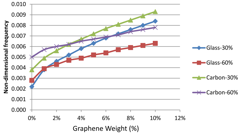
Fig. 6. Fundamental frequency vs. GPLs content for laminates with anti-symmetric stacking sequence [90/0/90/0]_{\text{anti-s}} , D/a = 0.03 , h/D = 0.125 , a/b = 0.71 and skew angle \alpha = 45^\circ .
