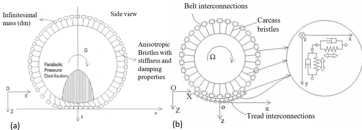
Figure 4: Various brush-type fundamental tyre modes [55, 57]
