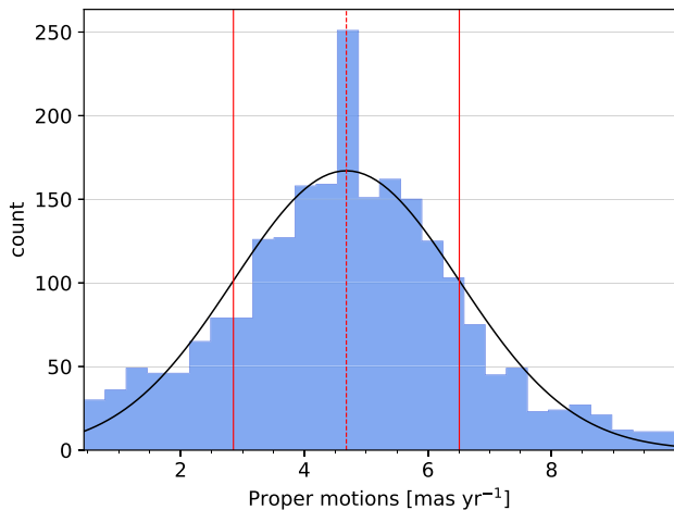
Figure 4. The galactic proper motion distribution for the 2240 OB stars identified in this study. We find a mean value of proper motion ( \mu ) = 4.68 \pm 1.83 mas yr ^{-1} to 1\sigma . Mean and 1\sigma limits are shown by vertical red lines.
