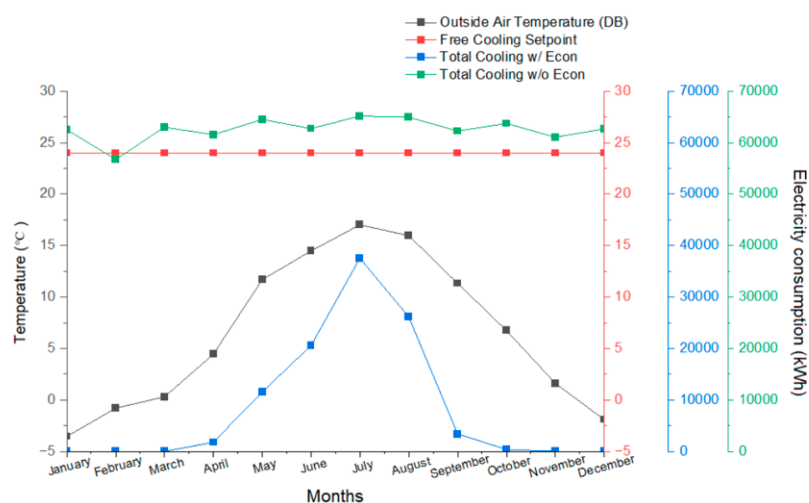
Figure 12. Stockholm outdoor air temperature electricity impact (economiser vs. no economiser).
