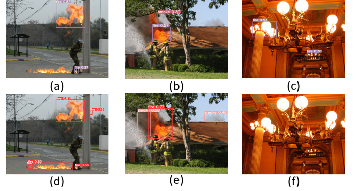
Fig. 5. Some predictions results from the BoWFire dataset [48], (a)-(c) are the results for the original YOLOv5 and (d)-(f) are the results for the proposed YOLOv5. The detection results show that the proposed YOLOv5 can mark out more areas where flames and smoke are present in the pictures and there are no false detections in pictures with flame-like objects.
