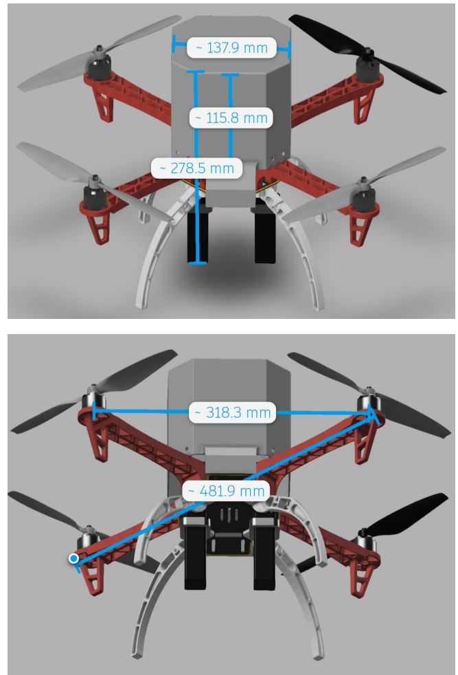
FIGURE 19: Shielded Maggy.
