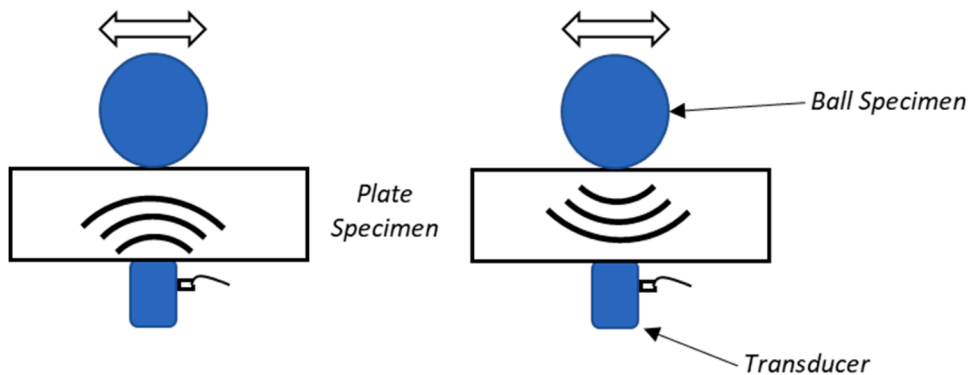
Fig. 7. Ultrasound sensing method (after [58]).
