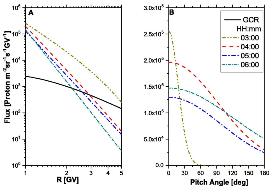
Fig. 51 Derived proton spectra and Pitch Angle Distribution (PAD) during GLE#70 using full neutron monitor modelling. Panel A and B show the reconstructed SEP spectra (the black solid line corresponds to GCRs) and PAD, respectively, for several stages of the event as denoted in the legend. During the initial stage close to 0300 UT the particles had small pitch angles, hence they are field-aligned. Modified after Koldobskiy and Mishev (2022)
