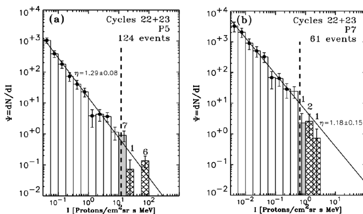
Fig. 8 Size distribution of SEP peak intensities from GOES proton channels P5 ( \sim 39\text{--}82 MeV, left) and P7 ( \sim 110\text{--}500 MeV, right) for data including solar cycles 22 and 23 (reproduced from Lario et al. 2008). The vertical dashed lines indicate the proposed streaming limit
