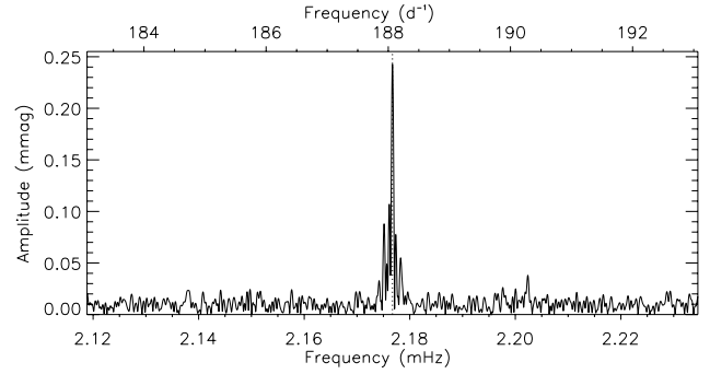
Figure 3. Amplitude spectrum of TIC 165052884 with the pulsation mode identified by the vertical dotted line.
