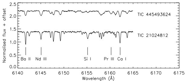
Figure A2. HERMES spectra of TIC 445493624 and TIC 21024812 in the red region.
