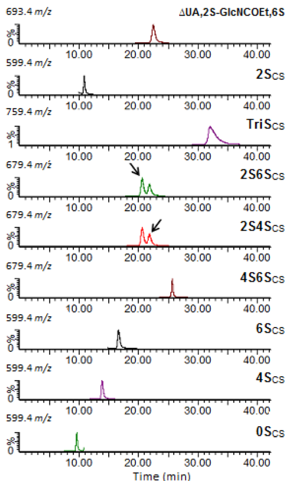
Fig. 3 SIR chromatogram of procainamide-labelled CS disaccharides and internal disaccharide standard ( 20 \mu\text{g mL}^{-1} each) using optimum MS conditions. The monitored MS ion for each disaccharide is also shown.
