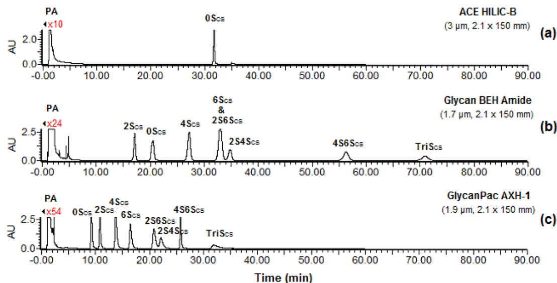
Fig. 1 LC separation of procainamide-labelled CS disaccharides using HILIC columns (a) ACE HILIC-B (b) glycan BEH amide and (c) GlycanPac AXH-1. Mobile phase A, B and C was ammonium formate (pH 4.4), acetonitrile and water respectively. Detection was diode array, and a wavelength of 299 nm was used for extraction of chromatograms. PA (procainamide peak).
