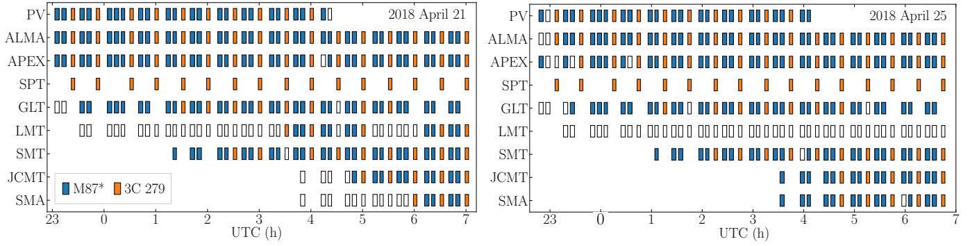
Fig. 3. EHT observing schedules for M87* (blue) and its calibrator 3C 279 (orange) on the 2018 April 21 (left panel) and April 25 (right panel) observing days, which began at the end in UTC of April 20 and 24, respectively. Open rectangles represent scans that were scheduled but not observed owing to weather or technical issues. The filled rectangles mark the scans with detections in the final data set. On these two particular days, scan durations are typically 4 to 5 min each for M87* and 4 min each for 3C 279, as reflected by the width of each rectangle.
