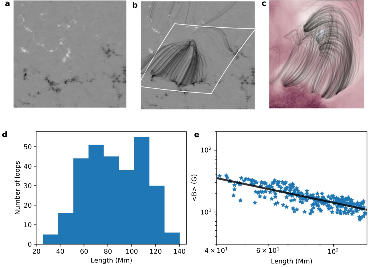
Figure 2. Panel (a) shows the HMI magnetogram projected onto an observer LOS of 50^\circ latitude and 30^\circ longitude. Extrapolated loops are overplotted on the magnetogram in panel (b). The white box represents the FOV of XBP-1 as shown in Figure 1. Panel (c) shows the projected extrapolated loops from the Sun–Earth LOS, on top of the AIA 211 Å image. Panels (d) and (e) show the distributions of 300 extrapolated loop lengths and the average magnetic field as a function of their lengths. The black line in panel (e) shows the \langle B \rangle \propto L^{-1} relation for reference.
