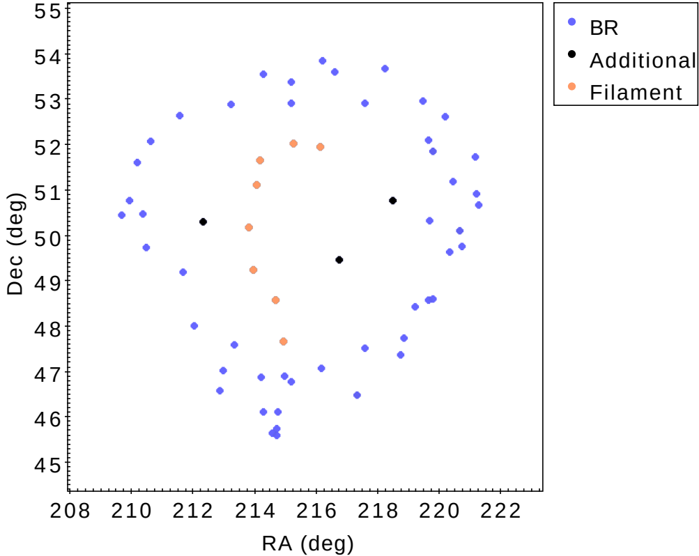
Figure 2. The Mg II absorbers in the visually-identified BR (blue), the inner filament (orange), and the additional absorbers inside the BR (black) from the on-sky perspective. Three of the blue points (BR) correspond to two absorbers occurring in one spectrum (see figure 8).
