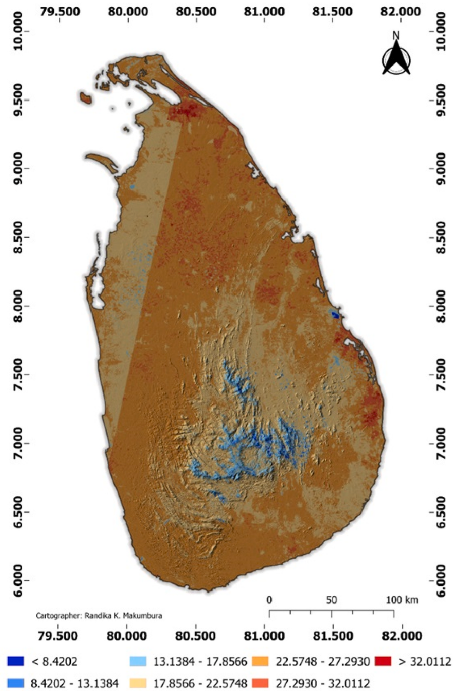
Fig. 6. Spatial variation of Land Surface Temperature (LST) for Sri Lanka in 2020.
