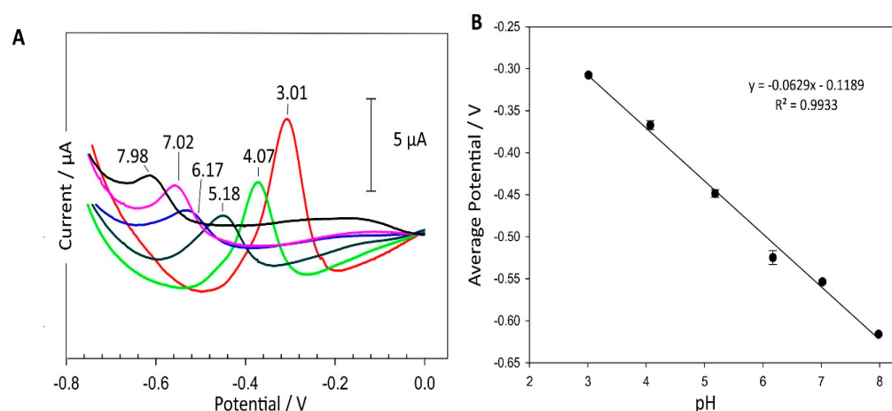
Figure 6. (A) Square wave voltammograms detailing the response of a two-electrode riboflavin-modified carbon fiber 3D-printed hub to BR buffers of varying pH. (B) Associated regression data. Note: Each point relates to the average of 5 scans and error bars represent the mean standard deviation. Responses were recorded using an integrated solid state ( 0.1 \text{ M KCl} ) \text{Ag} | \text{AgCl} pseudo reference.
