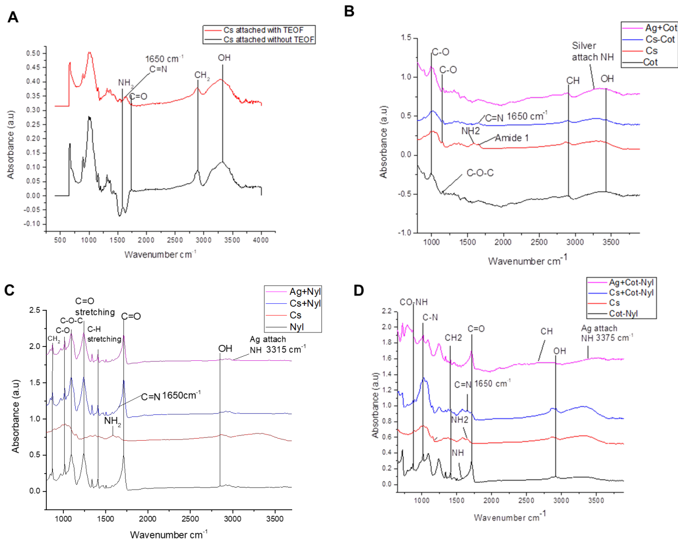
Figure 3. FTIR spectra of developed smart fabrics. A. Confirmation FTIR spectra of TEOF role in chitosan crosslinking with fabric. B. FTIR spectra of cotton fabric and its modifications. C. FTIR spectra of nylon fabric and its modifications. D. FTIR spectra of cotton-nylon fabric and its modifications.
