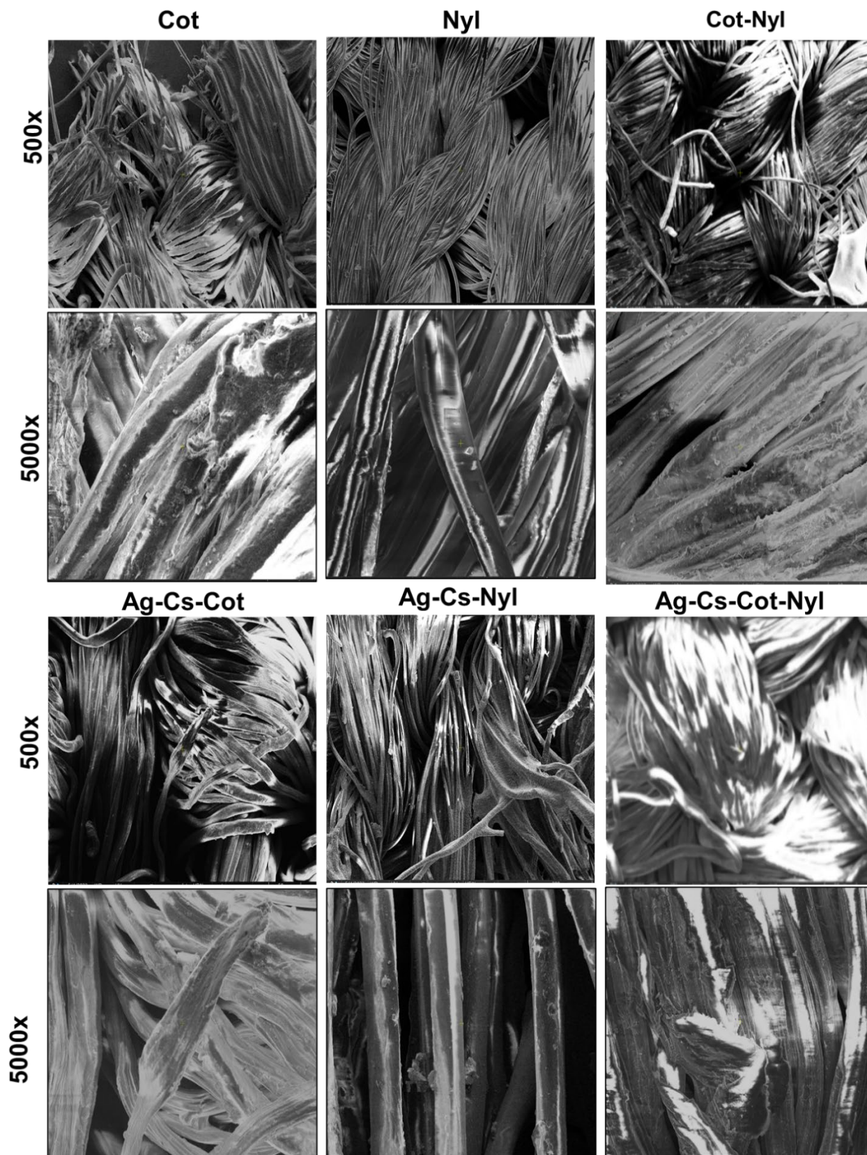
Figure 5. SEM images of plain and NPs loaded fabrics at 500X and 5000X.
