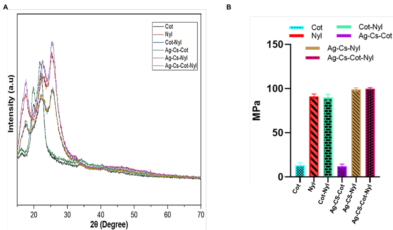
Figure 4. A. XRD spectra of synthesized smart fabrics. B. Tensile strength measurements of smart fabrics.
