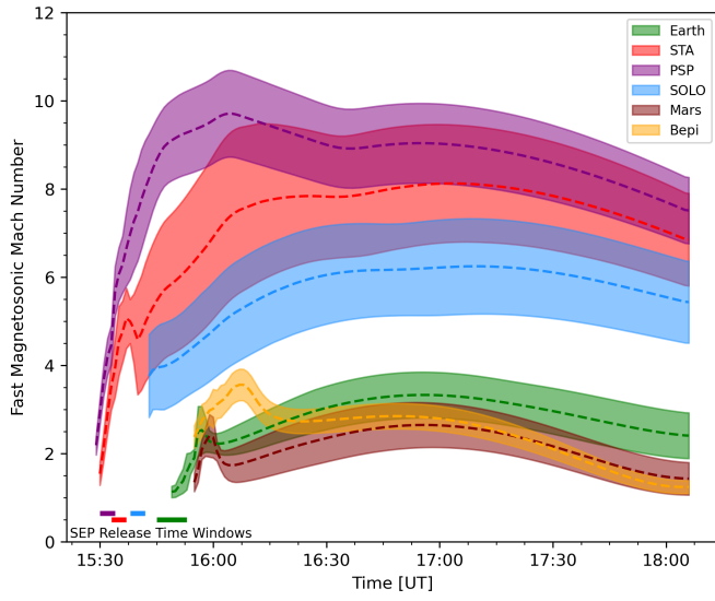
Fig. C.2. Similar to Figure 5. The colour-shaded areas depict the variation of M_{fm} using the PFSS connectivity estimates.
