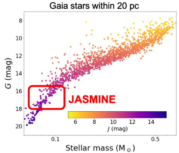
Fig. 13. Gaia G -band (y-axis) and 2MASS J -band (colors) magnitudes of the stars within 20 pc as a function of the stellar mass (x-axis). The UCD region to which JASMINE is sensitive to planets comparable to or higher than Gaia is indicated by the red box.
