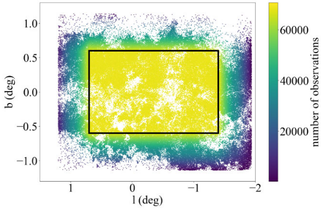
Fig. 16. Number of observations for each star observed towards the Galactic Center. The black rectangle highlights the JASMINE GCS field.
