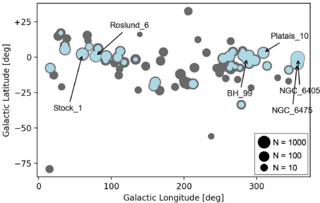
Fig. 9. Distribution of clusters that are closer than 500 pc from the Earth. The original list is cited from Cantat-Gaudin et al. (2018). The sizes of the data points represent the number of detectable cool targets within the FoV of 0^{\circ}.55 \times 0^{\circ}.55 , when transiting planets exist. The blue and gray colors correspond to assumed planetary radii of Earth size and Neptunian size, respectively. Details are described in subsection 3.3.
