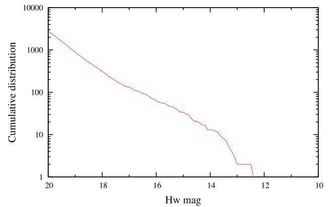
Fig. 22. Cumulative distribution of the H_w magnitude for asteroids observable throughout the JASMINE operation period.
