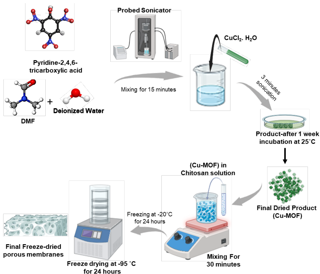
Figure 1: Synthesis scheme for preparation of Cu-MOF and Cu-MOF loaded chitosan membranes via Freeze drying method.
