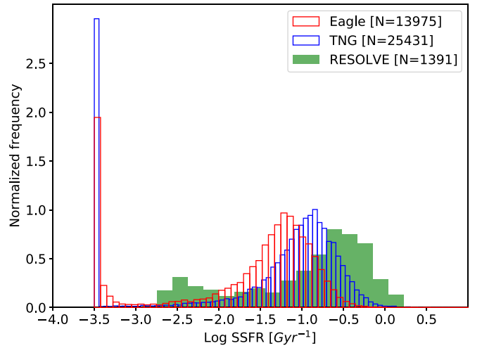
Figure 14. Distributions of sSFR for the RESOLVE survey (modified to use a floor of M_r \leq -17.33 in both subvolumes), IllustrisTNG simulation, and EAGLE simulation, where the simulations are also limited to M_r \leq -17.33 . Log sSFRs were truncated to -3.5 \text{ Gyr}^{-1} to avoid unphysical sSFR values from simulations. SF activity appears inconsistent between the three data sets.
