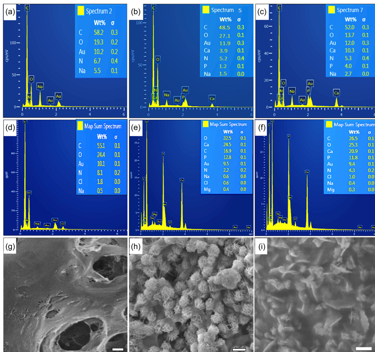
FIGURE 7 Energy dispersive spectroscopy (EDS) analyses of (a–c) hydrogels: CI, CII, and SI, respectively (scale bars are 1 \mu m) before simulated body fluid (SBF) treatment and (d–f) after 7 days of SBF treatment and (g–i) SEM images of those hydrogels treated in SBF for 14 days at their freeze-dried forms.
