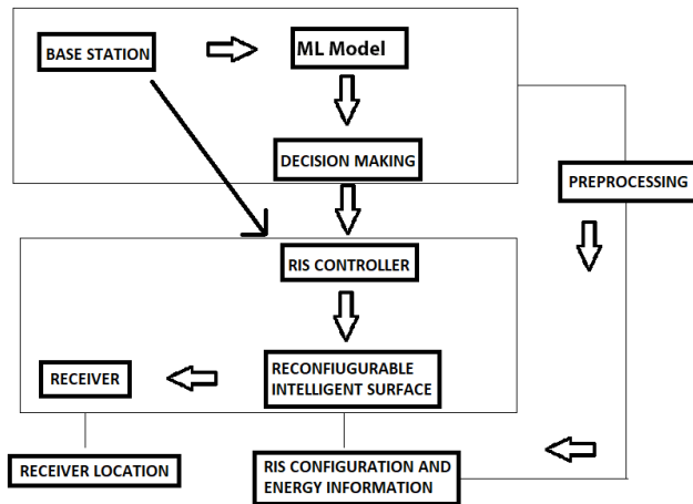
FIGURE 2. The system components architecture.
