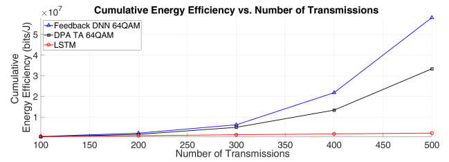
FIGURE 14. Cumulative Energy efficiency vs. Number of transmissions.
