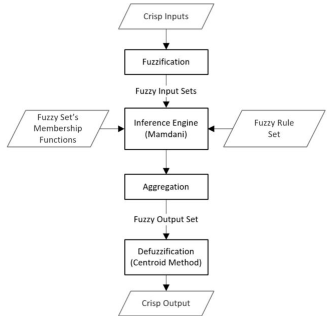
Fig. 4: Main processes of a fuzzy logic system [7], [8]. Fuzzification to determine fuzzy sets; inference engine to process the fuzzy input to the fuzzy output; defuzzification to map fuzzy sets into real-valued crisp variables.
