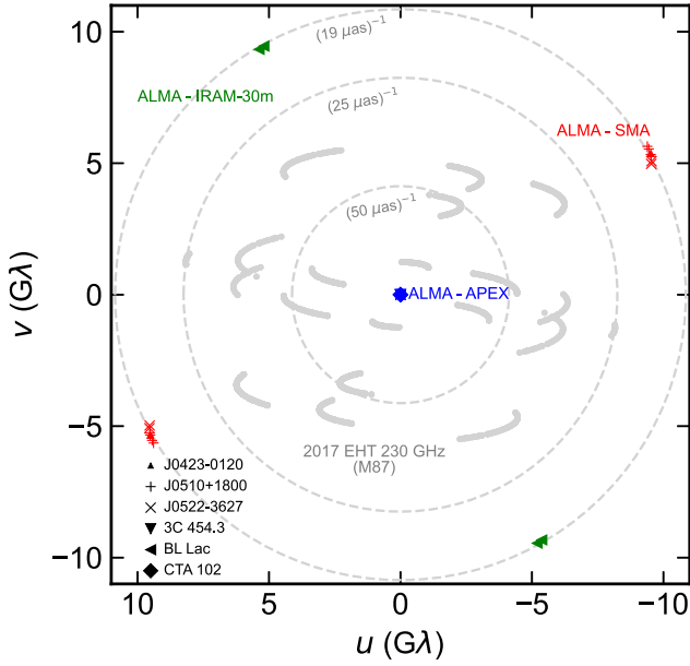
Figure 5. Detections on various targets at 345 GHz (see Table 1). The u-v locations of 230 GHz detections on M87* during the EHT 2017 April campaign are shown in gray including low-S/N scans at (25 \mu\text{as})^{-1} .
