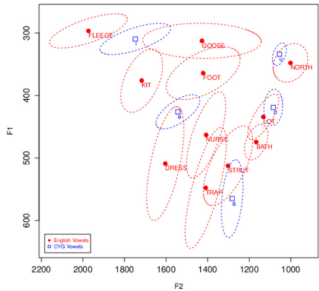
Fig. 10. F1x2 plot of English vowels produced by NE speakers and CYG vowels.
