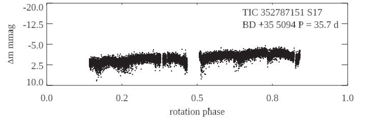
Fig. A.17. TIC 352787151 (BD +35 5094). S17 SAP data. Those have been phased with a rotation period of P_{\text{rot}} = 35.7 \text{ d} . There is no convincing rotational variability seen in these SAP data. The small amplitude is plausibly instrumental.
