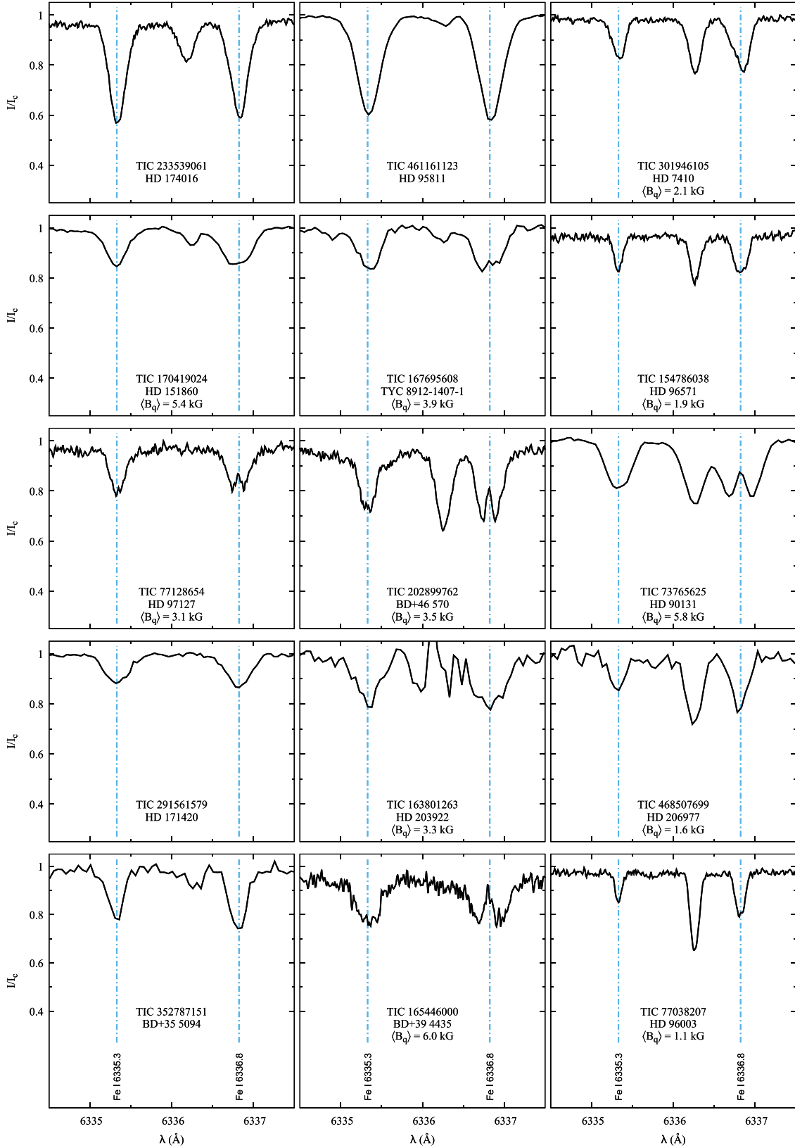
Fig. 5. Comparison of the profiles of the Fe I \lambda 6335.3 Å and \lambda 6336.8 Å lines as observed in the 15 stars of the present sample in which both are well visible. The spectra are shown in order of increasing effective temperature, from top to bottom, then from left to right. The value of the mean quadratic magnetic field \langle B_q \rangle is indicated at the bottom of each panel, for all stars in which its line broadening effect was above the limit of detection at the achieved spectral resolution. For those stars for which both HARPS-N and CAOS spectra were obtained, the \langle B_q \rangle value is the one determined from the higher resolution HARPS-N spectrum. The wavelengths are in the laboratory reference frame. The Zeeman patterns of the lines seen in the considered spectral range are illustrated in Fig. 6. The emission feature at \lambda \sim 6336 Å in the CAOS spectrum of HD 203922 is due to an instrumental glitch.
