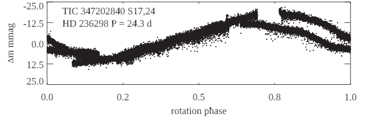
Fig. A.16. TIC 347202840 (HD 236298). Sectors 17 and 24 SAP data. Those have been phased with a rotation period of P_{\text{rot}} = 24.3 \text{ d} after some zero-point adjustments have been made. It is clear that there are further instrumental zero point shifts.
