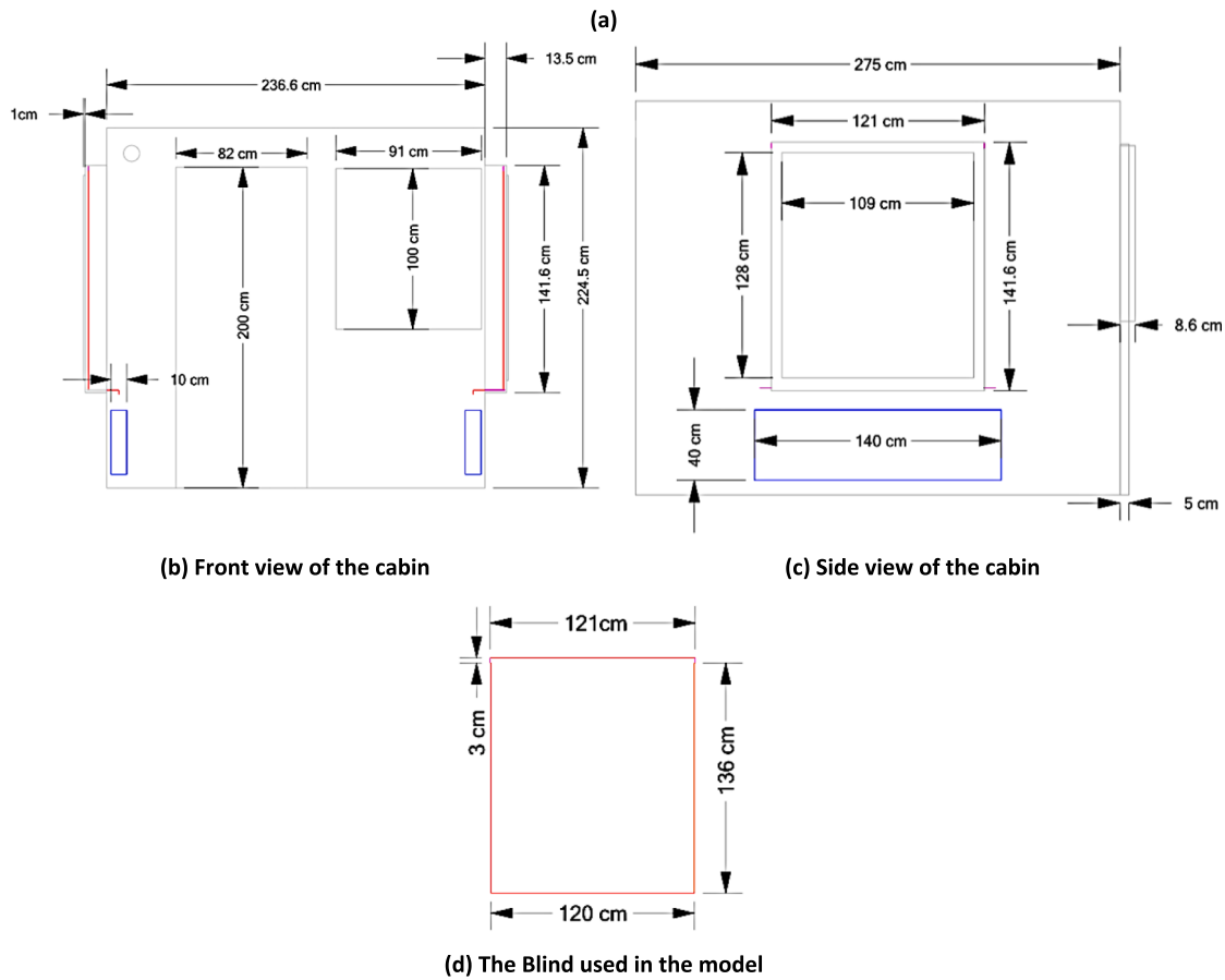
Fig. 3. (a) An employed CAD model for the computer simulation with details of different parts, (b–d) Dimensions of the test cabin and the main components,
