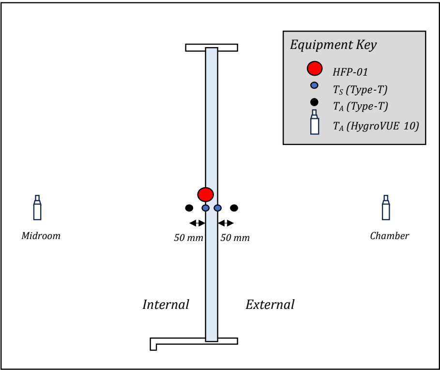
Fig. 6. Schematic diagram of sensors used for the analysis within this report.
