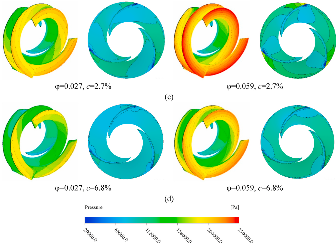
Fig. 6. (a) The distributions of the liquid water velocity for c = 2.7\% and (b) 6.8\% , and (c) comparison of the static pressure distributions of blades for c = 2.7\% and (d) 6.8\% at \phi = 0.027 and \phi = 0.059 for 2500 rec/min.
