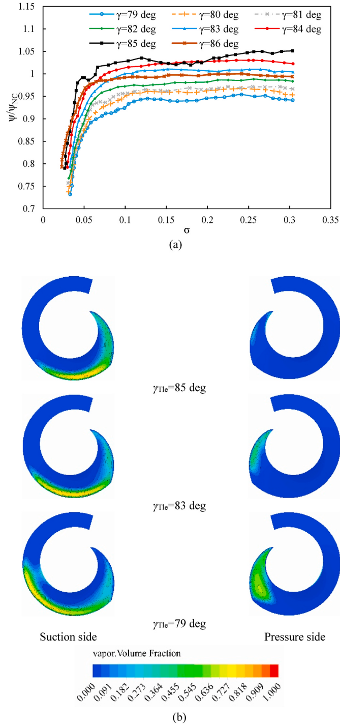
Fig. 11. (a) Effect of inlet tip blade angle on inducer cavitation performance, and (b) comparison of vapour volume fraction for different inlet tip blade angles at suction side and pressure side of inducer blades.
