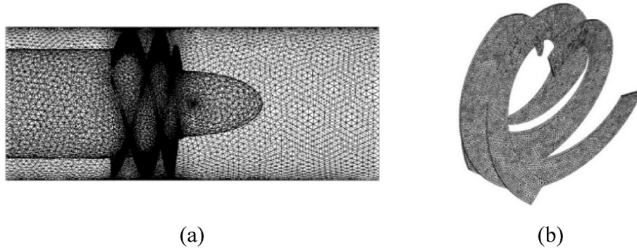
Fig. 3. The free grid of the entire computational field, including (a) the blade and (b) the inducer.
