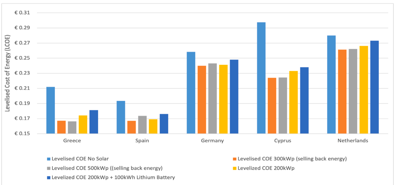
Fig. 6. Levelized Cost Of energy of different scenarios in different European countries.
