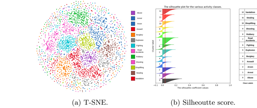
Fig. 5: (a) T-SNE plots for the BPTubeFormer models on the HRC dataset. (b) Silhouette plot for the classifications of the BPTubeFormer model on the HRC dataset. The y axis labels indicate the activity class labels. The red line indicates the average silhouette score for all the classes.
