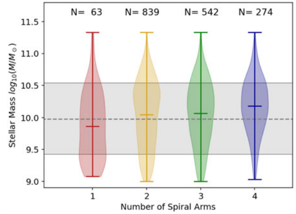
Figure 19. The distribution of stellar mass as measured by MAGPHYS vs the number of spiral arms for the GAMA galaxies with DESI-GZ ZOOBOT predictions classifications.
