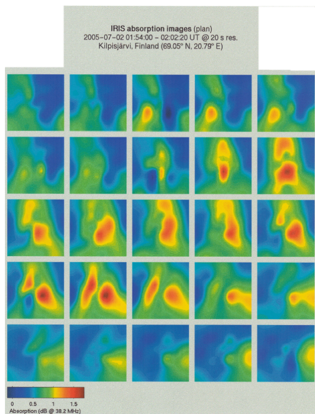
Fig. 11. The morning peak at 01:57 UT at 20 s resolution, over the period 01:54:00 to 02:02:20 UT. The field of view covers 240 km north-south and east-west, and is presented as if viewed from above.
