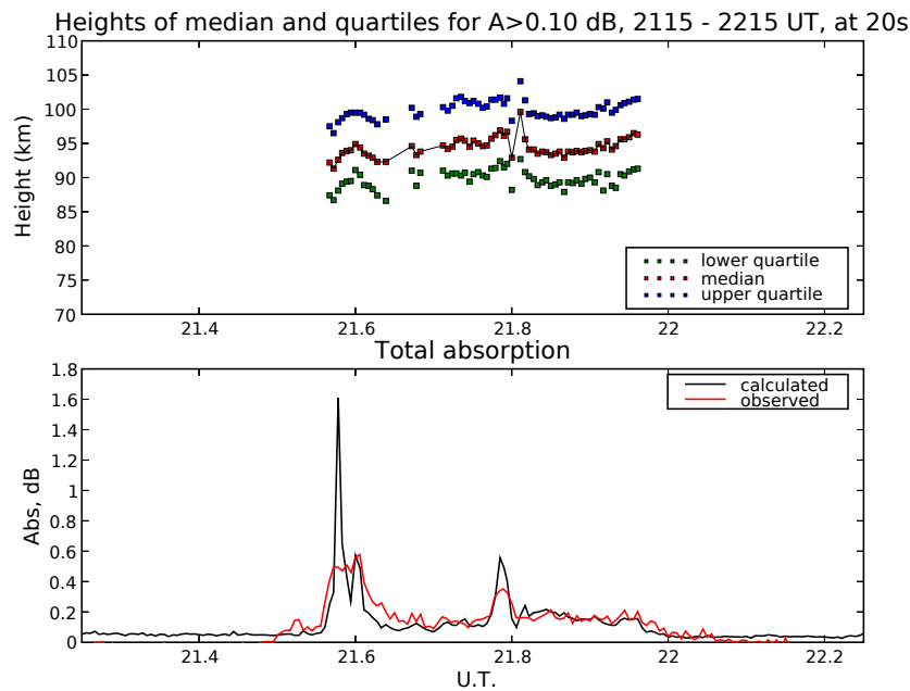
Fig. 7. Above: Heights of medians and quartiles for the absorbing region during the evening event of 1 July. Below: Total 38.2 MHz, calculated and observed.
