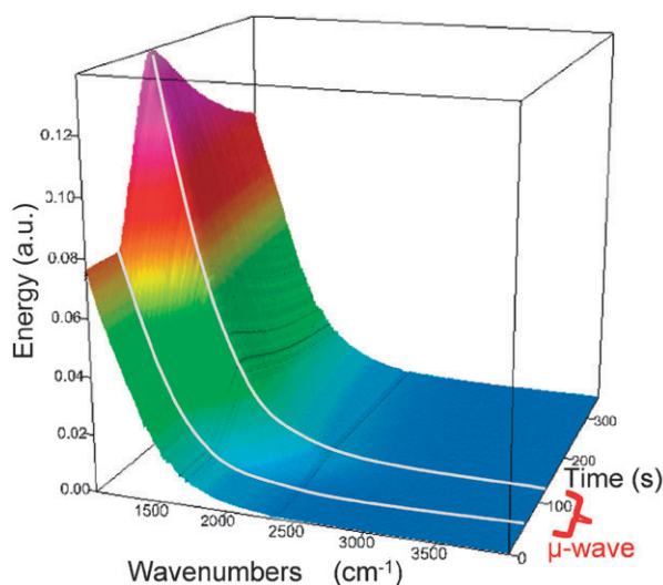
Fig. 6 Left: emission spectra of alumina during microwave irradiation. Right: temperature obtained by the black body law.
