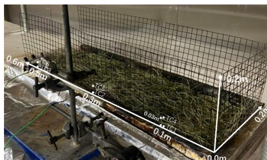
Figure 1 Medium scale experiment setup.
