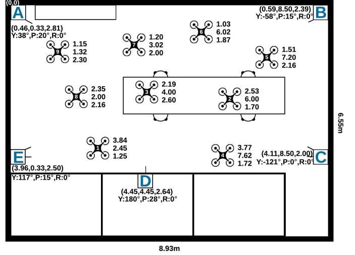
Fig. 1. mmWave and UWB 3D Positioning Experimental Setup (Y: Yaw, P: Pitch, R: Roll)
