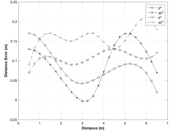
Fig. 2. UWB vs mmWave Precision Analysis
