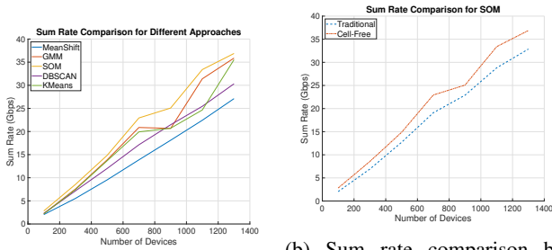
(a) Sum rate comparison for different approaches. (b) Sum rate comparison between traditional and cell-free networks.
