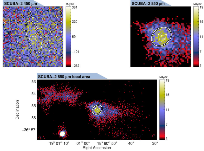
Figure B1. Example getsources output for a starless core. We show SCUBA-2 images at 450 and 850 \mu\text{m} . We also show a local area cut-out using the 850 \mu\text{m} data. Ellipses represent the estimated major and minor FWHM sizes of the core at each wavelength. If a core is significantly detected at the respective wavelength, the line is solid, and is dashed otherwise. We provide a complete set of these images for our dense cores.
