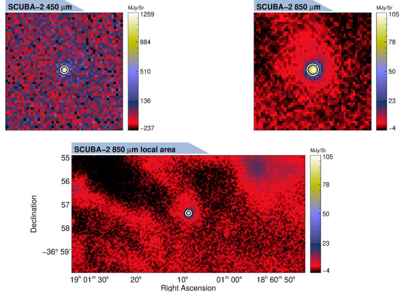
Figure B2. As Fig. B1, but for a protostellar core. The same image cut-outs are shown.
