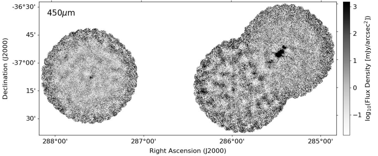
Figure A2. The reduced SCUBA-2 450 \mu\text{m} flux density map, shown in logarithmic scaling.
