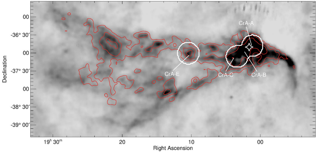
Figure 1. Finding chart of the Corona Australis molecular cloud. The background image shows IRAS 100- \mu m emission (Miville-Deschênes & Lagache 2005). The overlaid red contours show A_V extinctions of 0.5, 1.0, 2.0, and 5.0 mag (Dobashi et al. 2005). The regions observed as part of the JCMT GBLs are shown as white contours. Four subregions are labelled where data were taken. The white star towards the west of the image, in the vicinity of CrA-A, is the location of the Coronet cluster (Taylor & Storey 1984).
