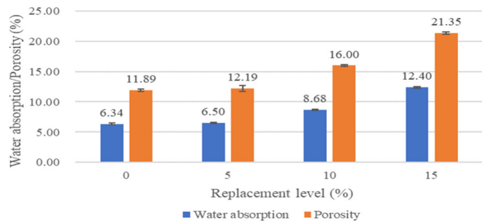
Fig. 5. Water absorption percentage and porosity of mortar at 28 curing days.
