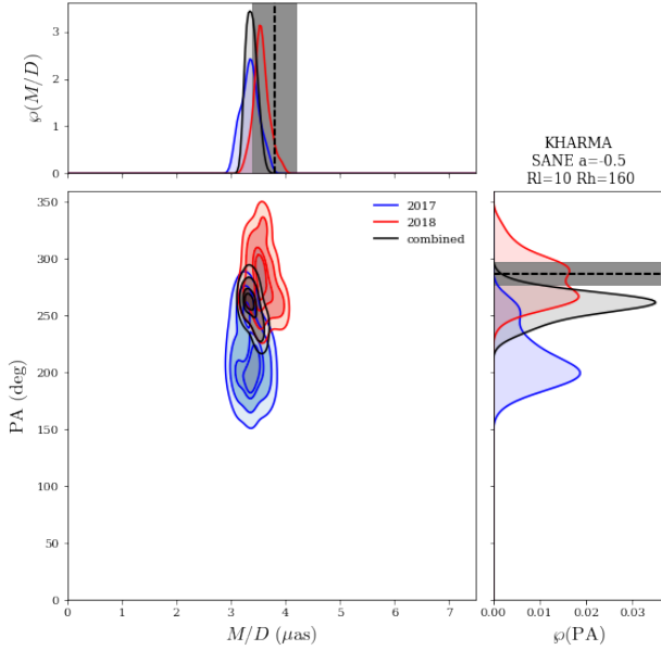
Fig. 6. Demonstration of the multi-epoch scoring based on the KCHARMA SANE model with (a_*, R_{\text{low}}, R_{\text{high}}) = (-0.5, 10, 160) . The 2017 and 2018 snapshot scoring results for the given model are shown in the M/D – PA plane with the blue and red distributions, respectively. The larger the overlap between the red and blue distributions, the better the fit of the multi-epoch observations with a single model. The black profile indicates the normalized combined distribution of the best-fit parameters computed according to the multi-epoch scoring procedure (see Sect. 4.4 for details). The dashed lines and shaded areas are the same as explained in Figs. 4 and 5.
