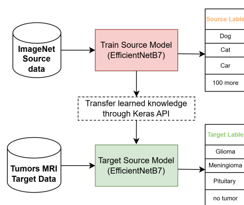
Figure 3. Adopted transfer learning method.
