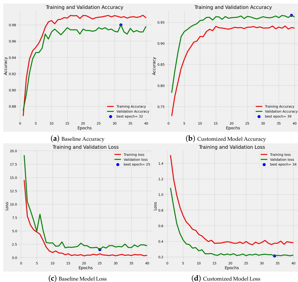
Figure 4. Accuracy and loss comparison between baseline and customized approach using small dataset BT_3264.
